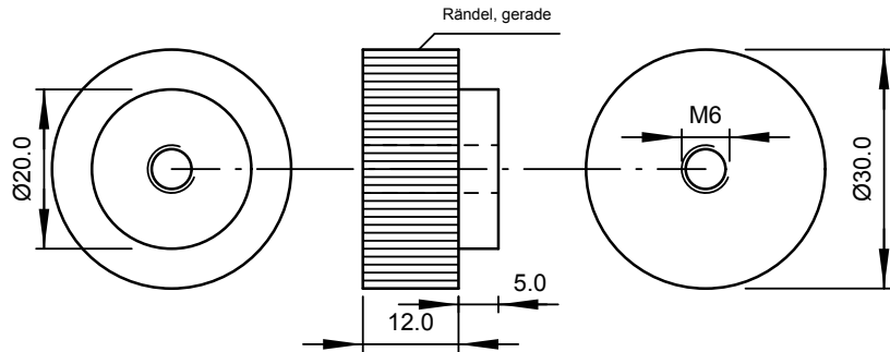
Handrad, Aluminium, (1x)
