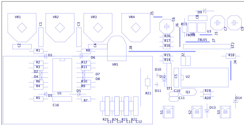
Drumtrigger Version 1 4 Channel Pad to Midi Converter (C) Stephan Asmus 10/2008
